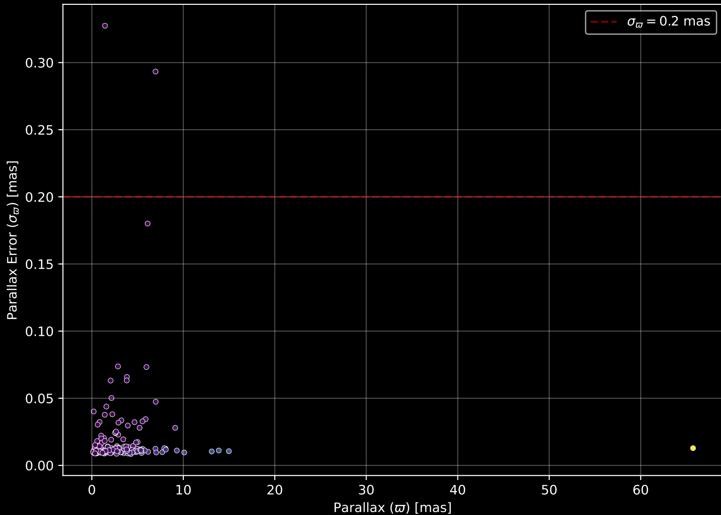
APOGEE DR17 Field: [268-25-O_TESS] Parallax Quality (n= 189)
