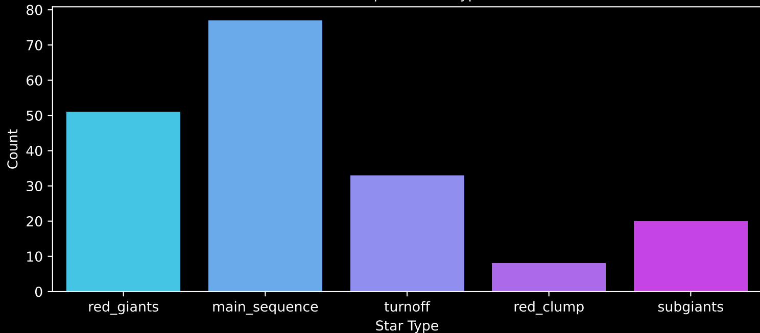
APOGEE DR17 Field: [268-25-O_TESS] Count plot of Star Type
