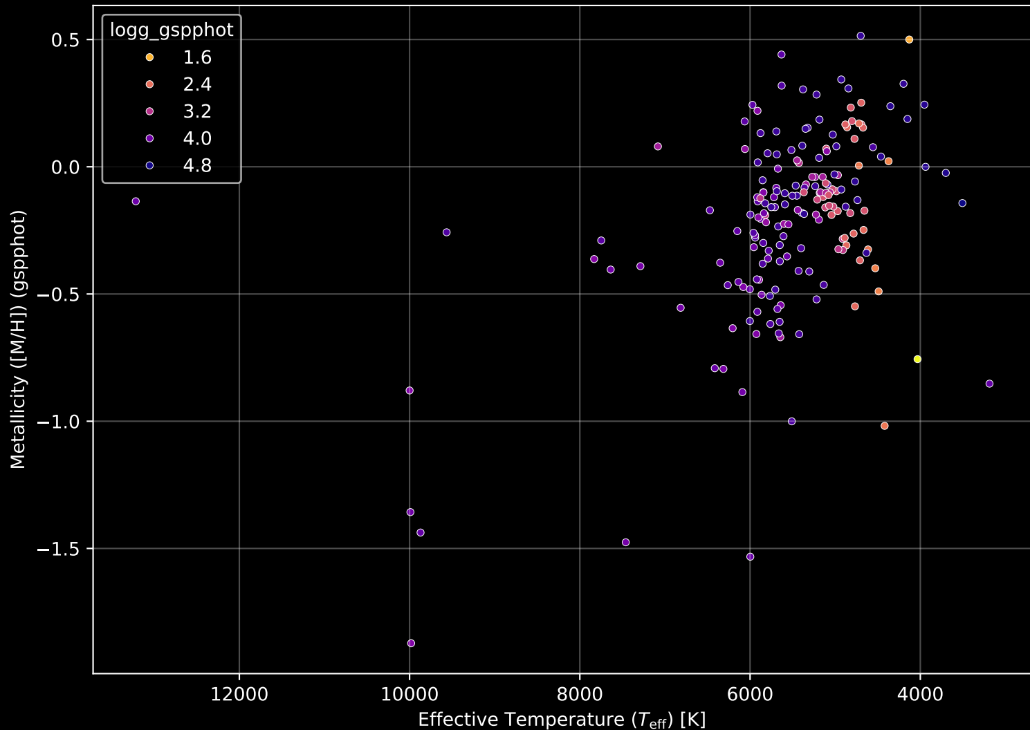
APOGEE DR17 Field: [268-25-O_TESS] Stellar Population Parameters (n= 189)
