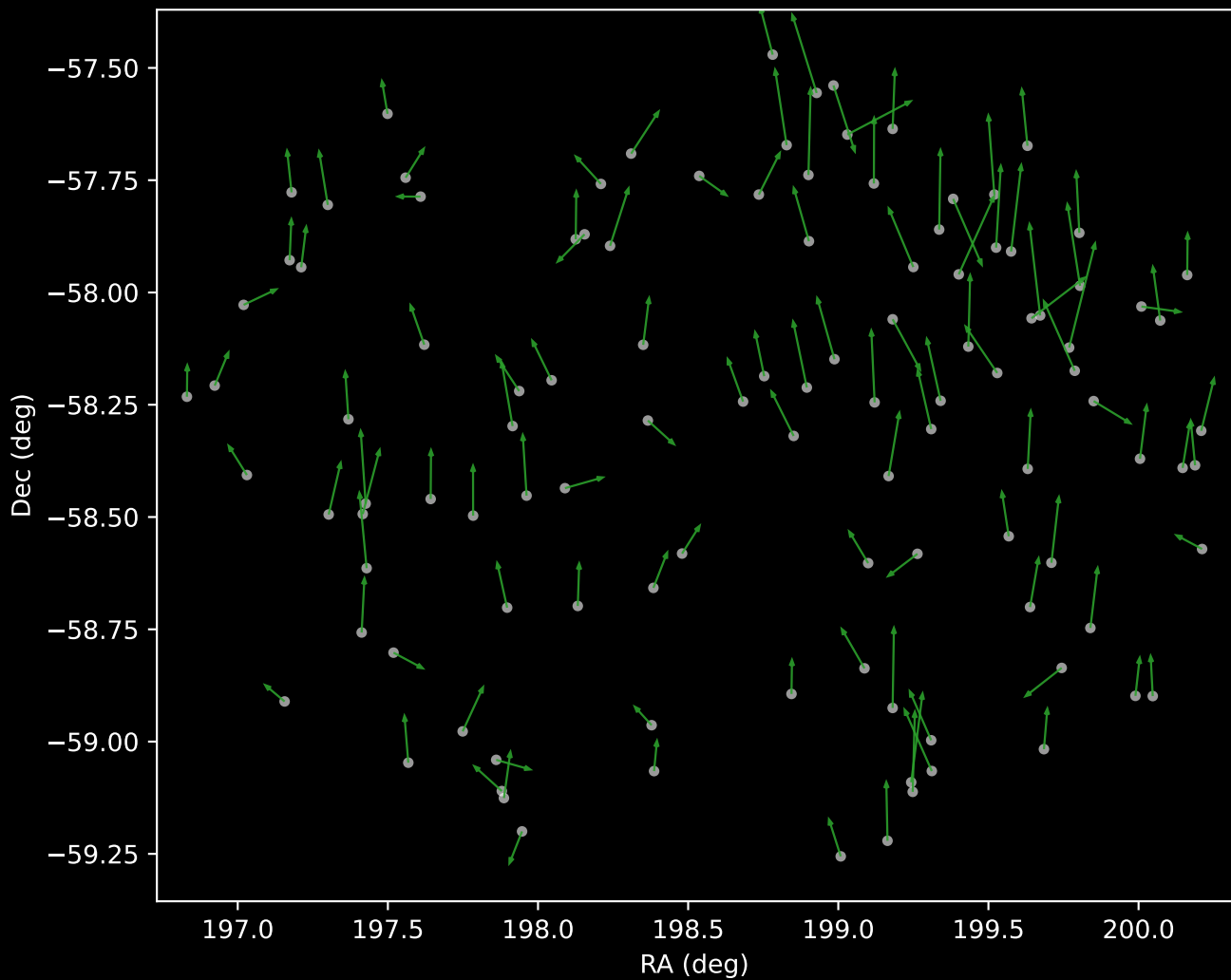
APOGEE DR17 Cluster 4 Proper Motion Vectors (n=112)
