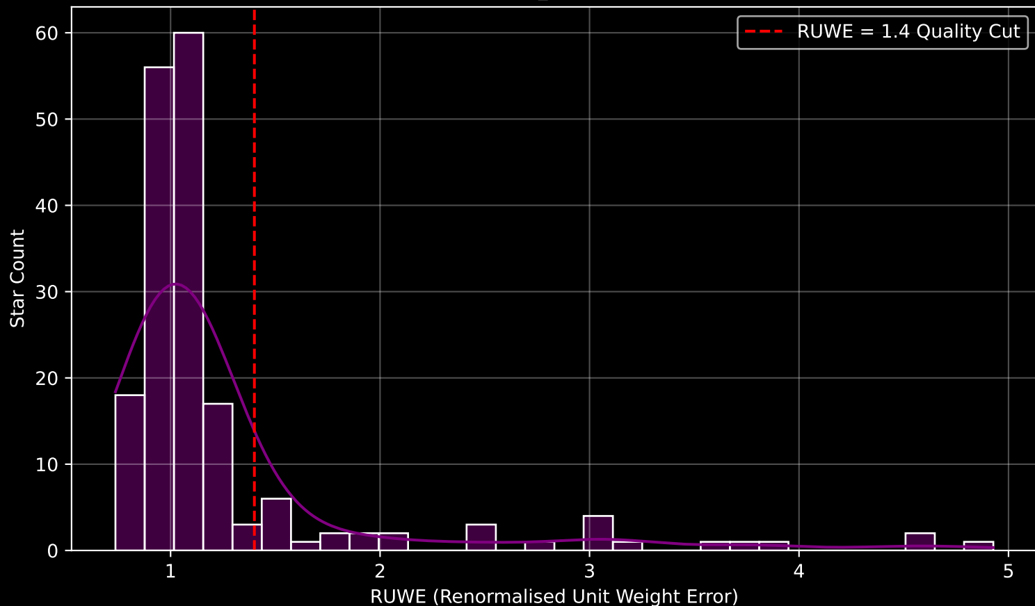
GAPOGEE DR17 Field [268-25-O_TESS] RUWE Distribution (n= 182)
