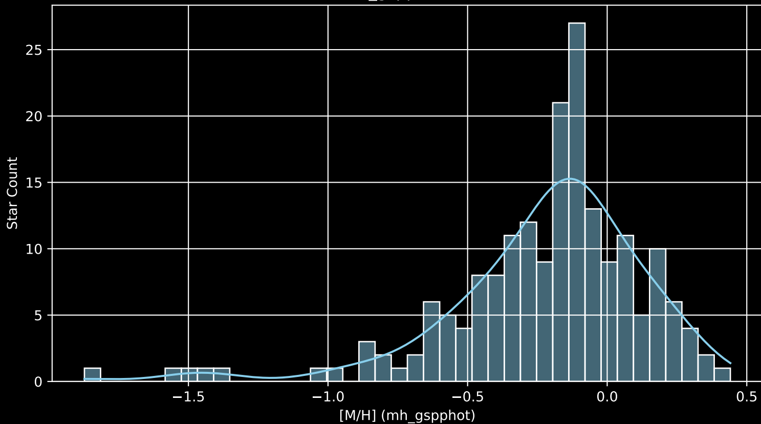
APOGEE DR17 Field: [268-25-O_TESS [M/H] (mh_gspphot) (n= 187)
