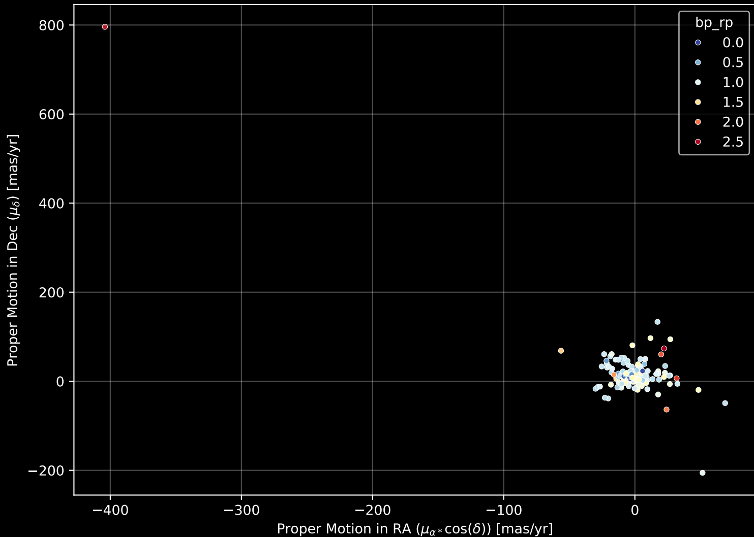
APOGEE DR17 Field: [268-25-O_TESS] Proper Motion Diagram (n= 189)
