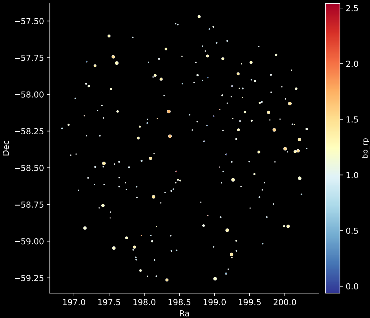
APOGEE DR17 Field: [268-25-O_TESS] Stars: 189
